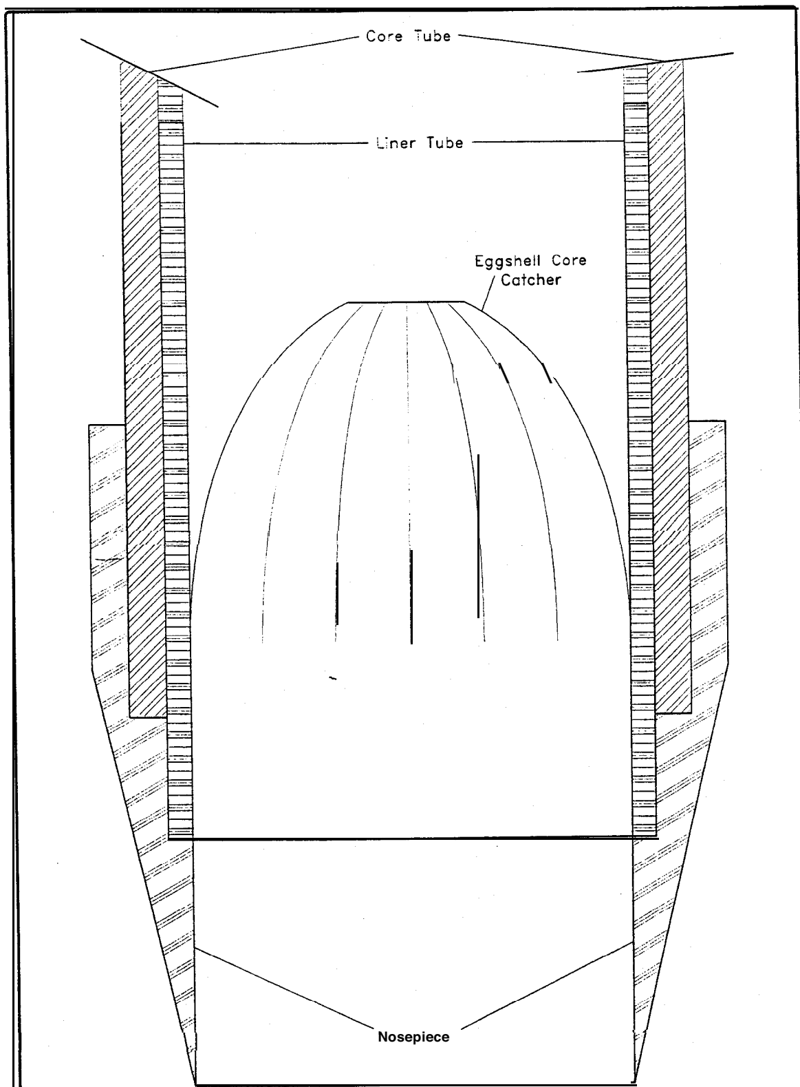
FIGURE IV: 3.4-i' Cross-sectional view of sediment sampler lower end (TAEM 1996).
