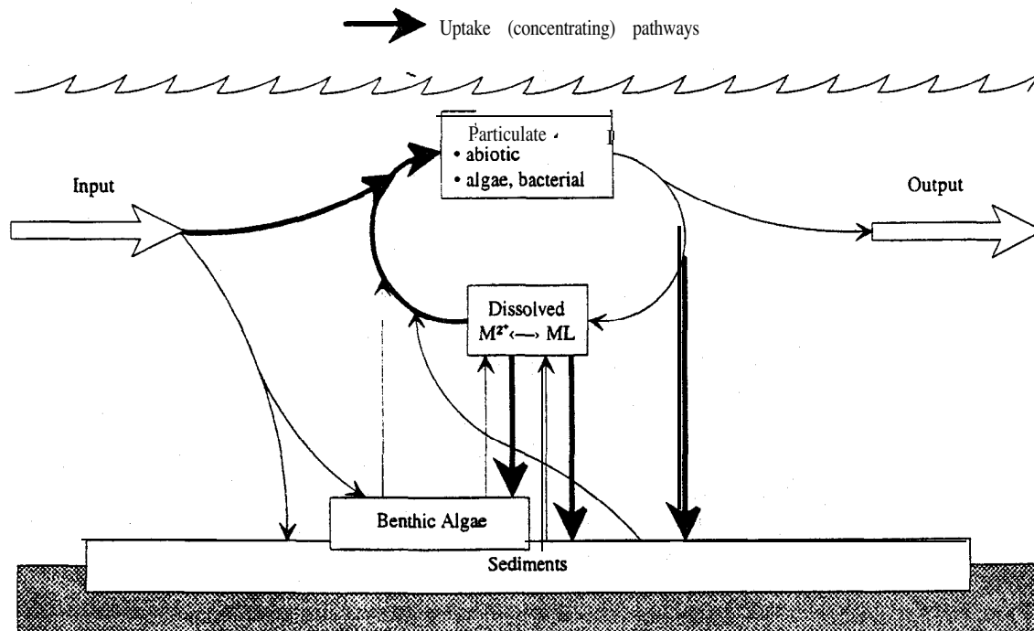
FIGURE IV: 3.1-Ib Simplified biogeochemical cycle for trace metals in fluvial systems including the interaction with benthic algae (Hart 1982).
