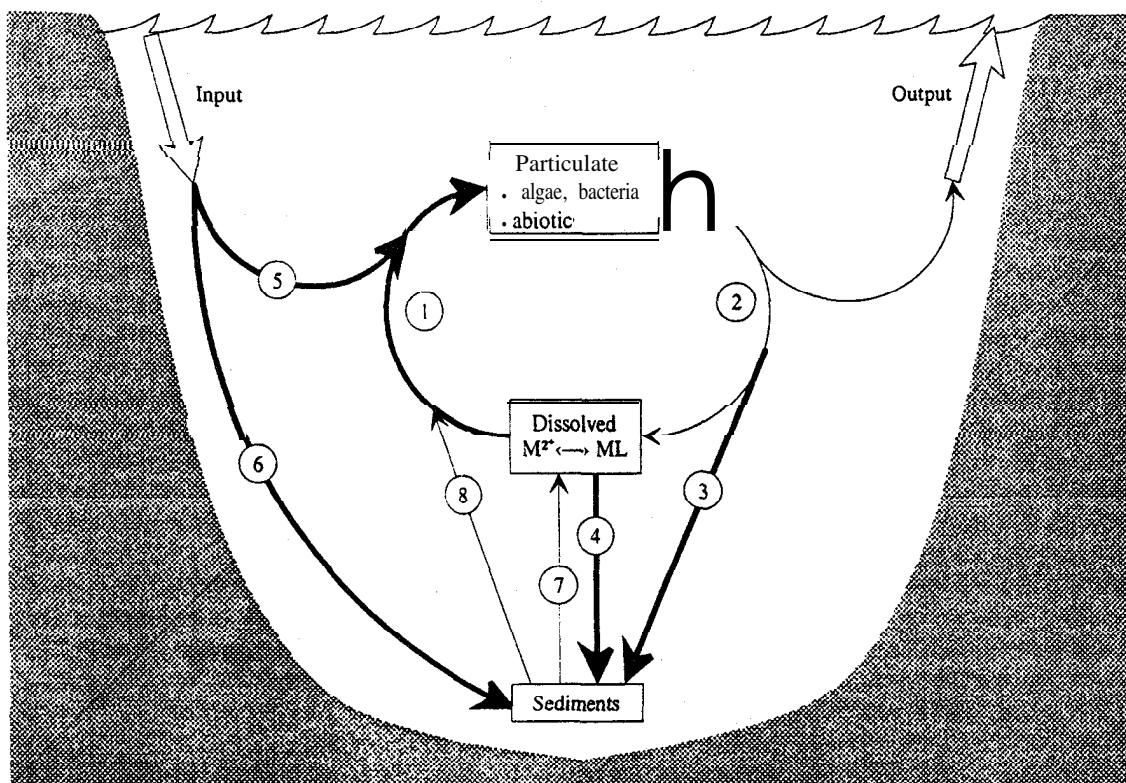
FIGURE IV: 3.1-Ia (1) see section IV: 3.1 For further details Simplified biogeochemical cycle for trace metals in lakes (Hart 1982).
