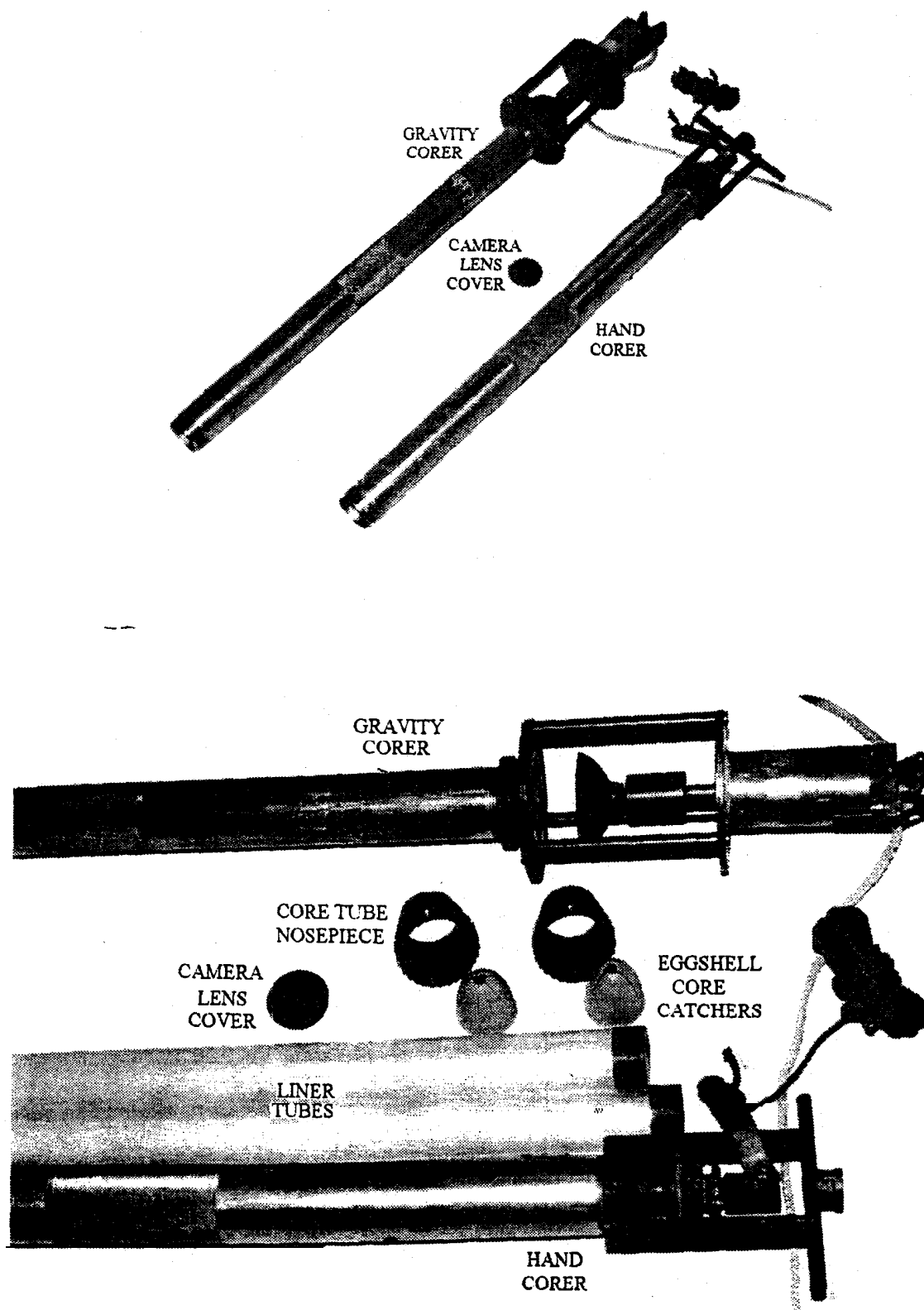
FIGURE IV: 3.4-6 Gravity and hand corers with accessories (TAEM 1996).
